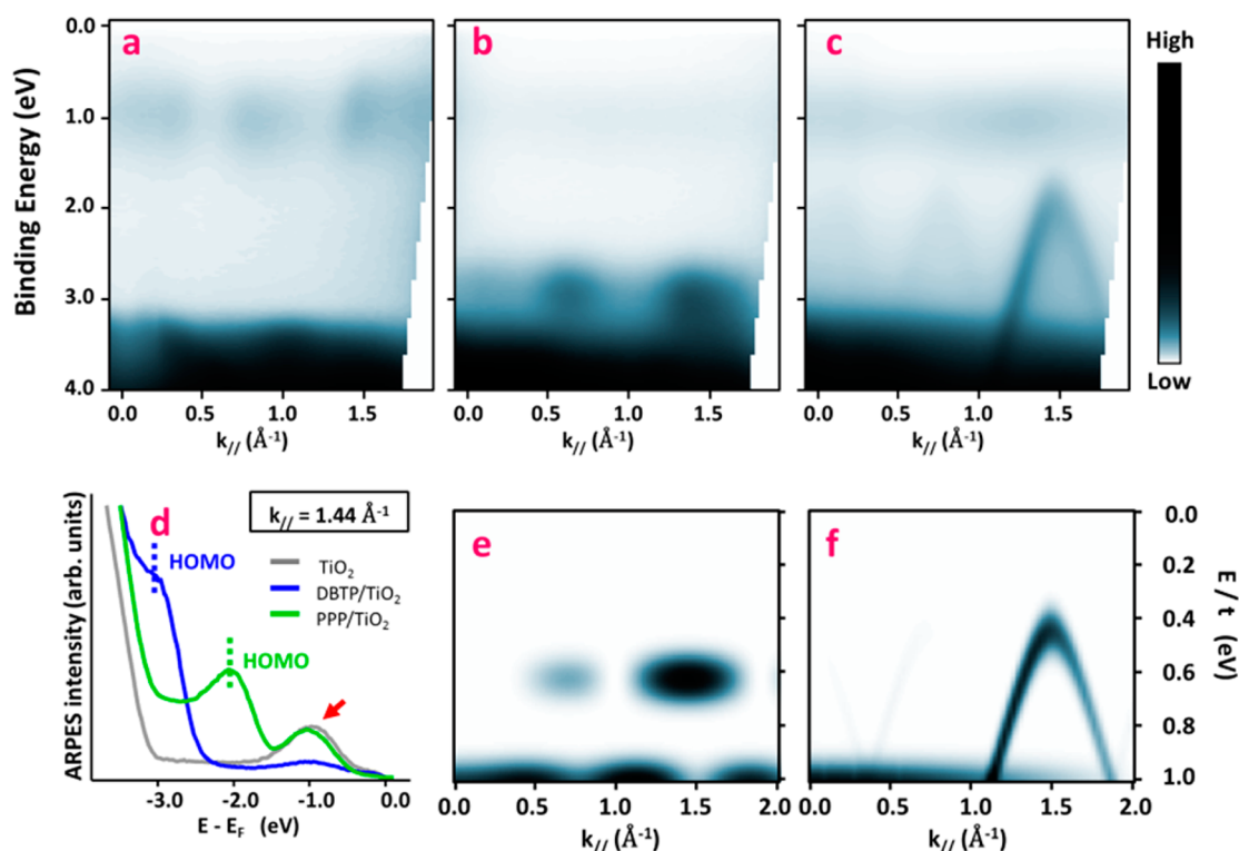
Figure 3. Angle-resolved photoemission spectroscopy: (a–c) experimental raw ARPES intensity maps acquired on the pristine surface (a), after 1 ML DBTP deposition at room temperature (b), and after 1 ML deposition with the sample kept at 575 K (c); (d) energy dispersion curves taken at k_{||} = 1.44 \text{ \AA}^{-1} from the three previous maps; (e, f) theoretical ARPES intensity distributions calculated within a tight-binding model for a terphenyl molecule (e) and an infinite poly( p -phenylene) chain (f). The energy scale ( E ) is normalized by the resonance integral ( t ) between the p_z orbitals of two neighboring carbon atoms.
